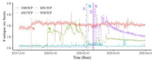
FIGURE 2. The number of unique source hosts per hour on NICTER where the malware activities were observed (December 2019 to March 2020). D: The earliest time detected by Dark-TRACER, N: The time observed by NICTER operators, and P: The time when it was revealed to the public.
