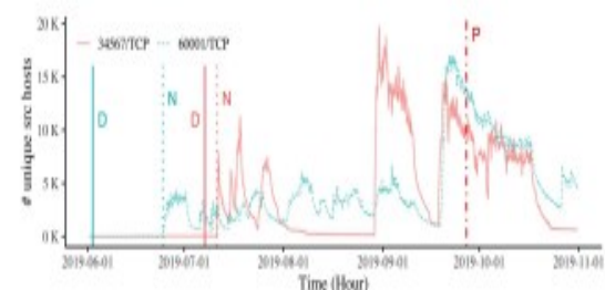
FIGURE 1. The number of unique source hosts per hour on NICTER, where Moonboot-related malware activities are observed. Here, the events that do not fluctuate synchronously
