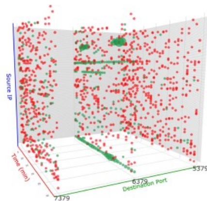
FIGURE 4. A 3D graph visualizing a case of anomalous synchronization of the spatiotemporal patterns detected from the experimental results in Section III. A scatter plot of partial Vmpp during 18:30–19:00 on October 31, 2018, is visualized. Each of the three axes is a time axis in minutes, a source-host spatial axis, and a destination-port spatial axis, and the plots represent the observed packets (element values in Vhp). For the destination-port spatial axis, there are only three points at which anomalous synchronicity was detected—5379, 6379, and 7379. Host IPs are plotted in red if they match on multiple ports within one-minute increments and in green if they do not. The red points are considered to be synchronized communications caused by factors such as malware activities, while the green points are considered to be noise communications.
